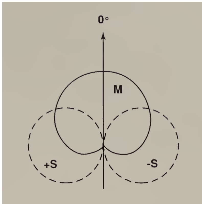
Figure 7.28: The basic configuration of a Mid/Side stereo pickup; the mid microphone is aimed at the 0^\circ axis. The side microphone is a bidirectional, with its null plane aligned with the principal axis of the mid microphone. By convention, the positive lobe of the side microphone is oriented to the left side of the stereo soundstage. Reproduced from Streicher R, Everest FA; 1998. 73(fig7.17)
