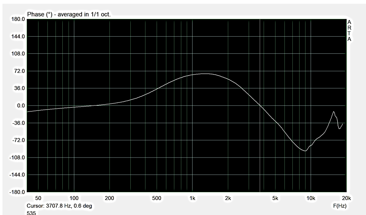
Figure 7.9: Earphone #2 phase estimate
