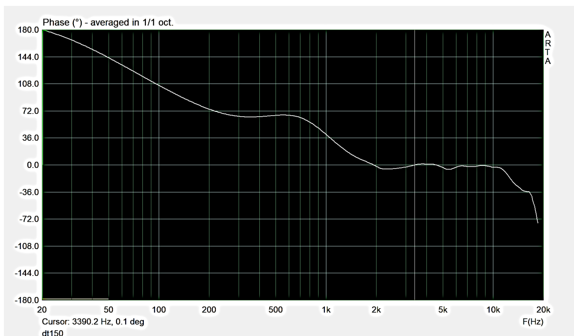
Figure 7.11: Earphone #4 phase estimate
