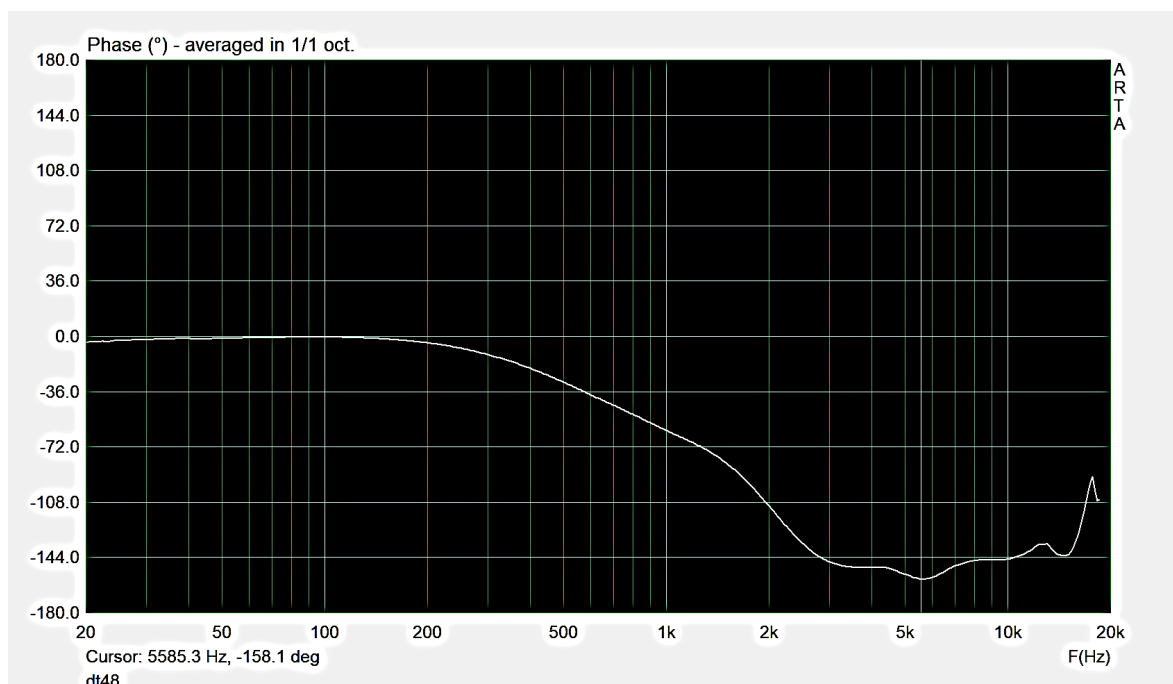
Figure 7.10: Earphone #3 phase estimate
