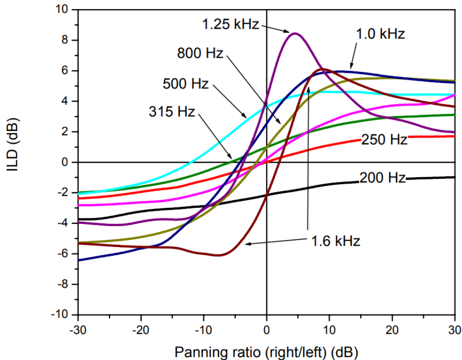
Figure 3.3: ‘ILDs for a [typical] listener and 60° stereo triangle’. 187(fig19) Reproduced from Benjamin E, 2006.
