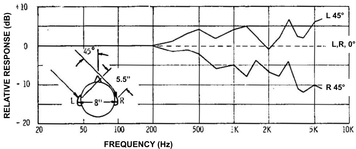
Figure 2.3: Reproduced from Bauer BB, 1961, 69(fig3) a graph prediction of relative responses at the left (L) and right(R) ears from a loudspeaker positioned at 45° horizontal orientation, derived from Wiener 70 . The “head-on” function (L,R, 0°) is shown as relatively flat. Note between the ear dimension as 8 inches (203 mm), and approximated increased path-length to right ear of 5.5 inches (140 mm). It may be assumed that the common recommended stereo loudspeaker arrangement of \pm 30^\circ had yet to be realised until a decade or more later. 71(p127),72
