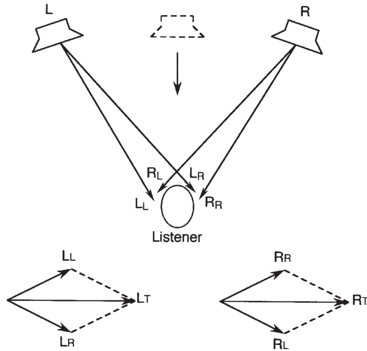
Figure 2.2: Two loudspeakers reproducing the same programme content creating equal net phasors, below 700 Hz, at both ears – reproduced from Eargle J, 2004. 61(figs11-2) The equal phasors result in a phantom centre image in front of a forward-facing listener. L_L is the signal vector at the Left ear from Left loudspeaker, L_R is the crosstalk signal vector at Left ear from Right loudspeaker. L_T is vector addition of L_L and L_R , a forward phasor for partial contribution to a phantom centre image. Adapted from Bock TM, Keele, Jr. DB (Don); 1986. 62
