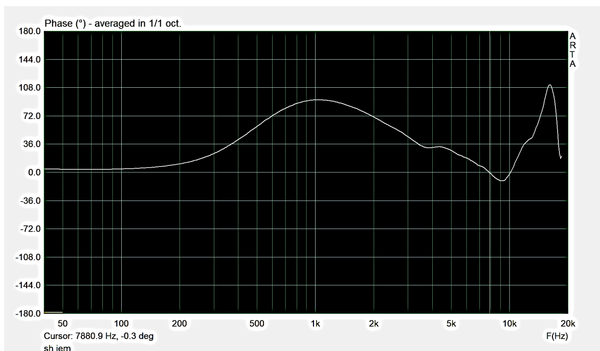
Figure 7.15: Earphone #8 phase estimate
