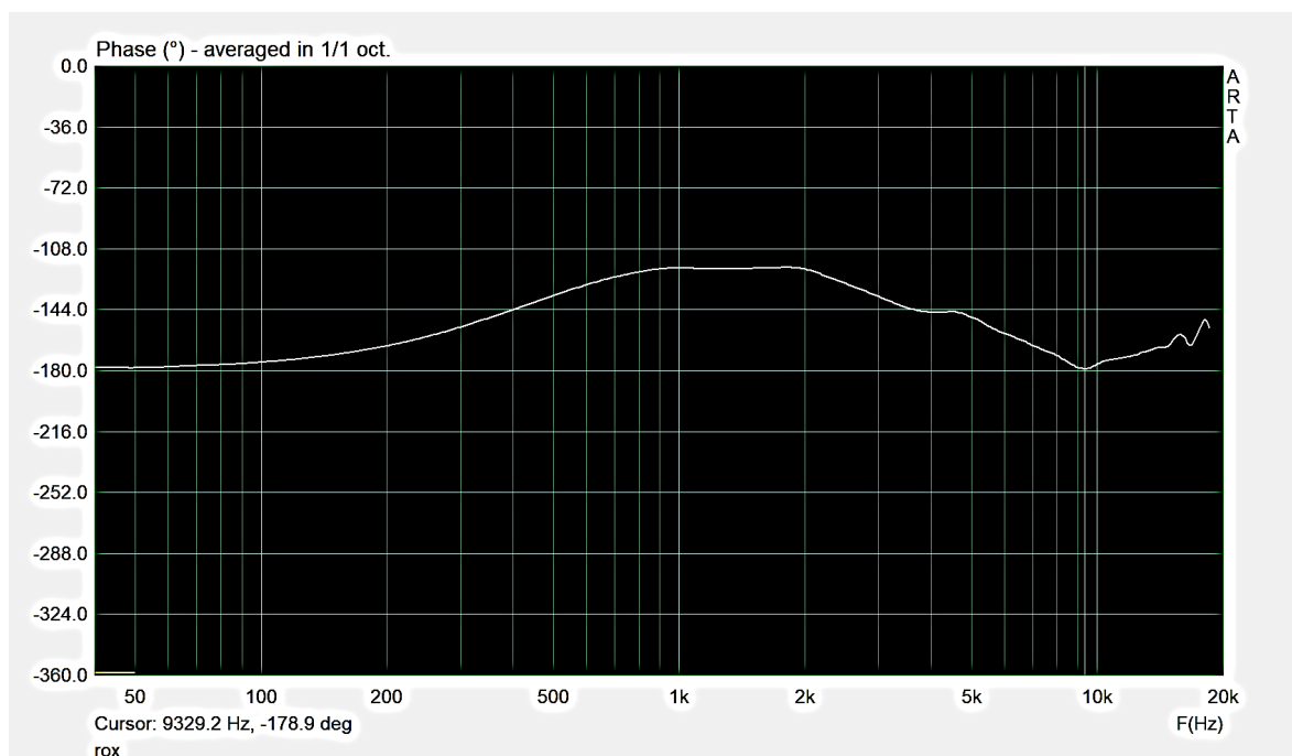
Figure 7.14: Earphone #7 phase estimate (note Phase range)
