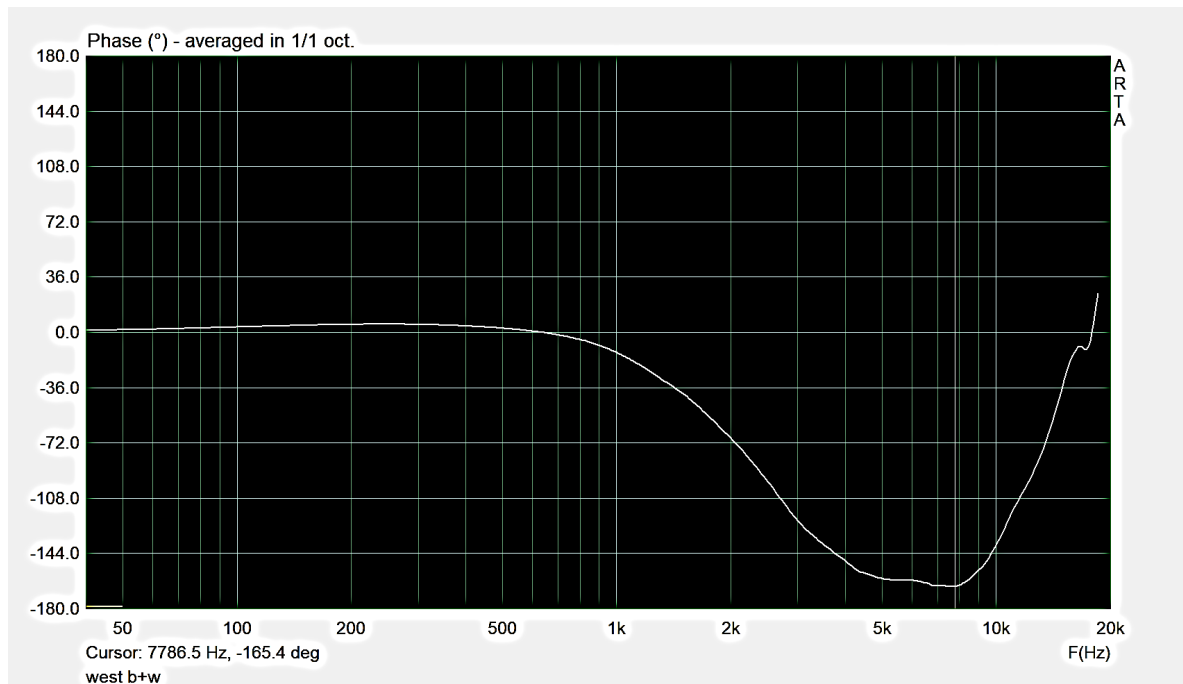
Figure 7.18: Earphone #11 phase estimate
