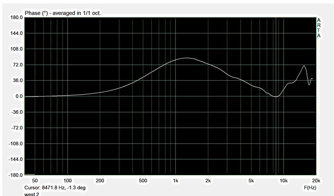
Figure 7.17: Earphone #10 phase estimate
