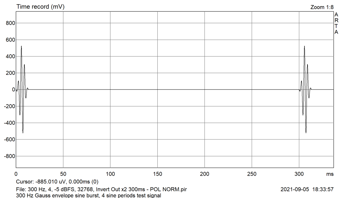
Figure 3.1: POL3 test signal, a 300 Hz Gauss envelope tone burst, 4 sine periods. Zoom 1:8
