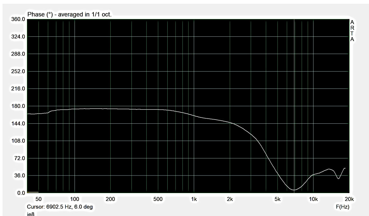
Figure 7.13: Earphone #6 phase estimate (note Phase range)
