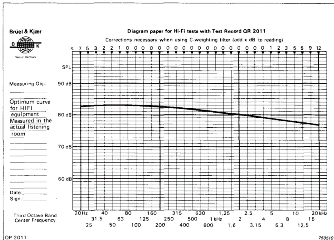
Figure 7.20: ‘Optimum curve for HIFI equipment. Measured in the actual listening room’. 93(fig5) Reproduced from Möller H, 1974.
