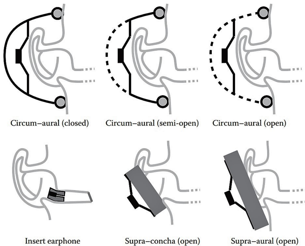
Figure 7.3: Diagrammatic Horizontal Sections Showing Types of Earphones. Reproduced from Kleiner M, 2013. 254(fig24.1)
