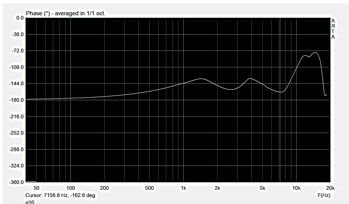
Figure 7.12: Earphone #5 phase estimate (note Phase range)
