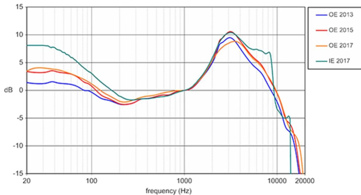
Figure 7.19: This graph compares the Harman curves published over the years, showing substantial variation in the bass and treble. Notably, the in-ear target [IE] reflects the difference in a blocked ear canal makes, as the blocked canal has it[s] own sets of resonances that the IEM needs to compensate for. (From: Harman). Note: OE — Over the Ear headphone; IE — In-Ear earphone. Reproduced from Ilkless, 2021. 256
