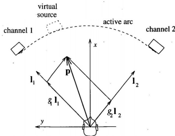
Figure 2.4: Stereophonic amplitude panning formulated with vectors: \mathbf{p} = \mathbf{g}_1 \mathbf{l}_1 + \mathbf{g}_2 \mathbf{l}_2 where \mathbf{l}_1 \mathbf{l}_2 are loudspeaker vectors; \mathbf{g}_1 \mathbf{g}_2 are the gains or amplitude levels for loudspeaker channel 1 and 2 . Altering the relative gains alters the virtual source position \mathbf{p} on the active arc. Reproduced from Pulkki V, 1997. 96(fig3)
