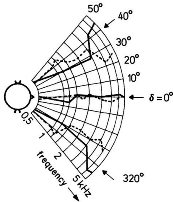
Figure 7.22: Direction of incidence of sound for sinusoids and Gaussian tone bursts of critical bandwidth so that the same direction of the auditory event is achieved as with broad band noise from the directions \delta = 0^\circ , 40^\circ , 320^\circ . Solid lines: sinusoidal signals (after Sandel et al. 1955 a sound pressure level 35 dB, 5 subjects, head immobilized). Dashed lines: Gaussian tone bursts (after Boerger 1965a b , b c ; 50-60 phon, 4-7 subjects, no head movement). Reproduced from Blauert J, 1996. 63(fig2.3)
