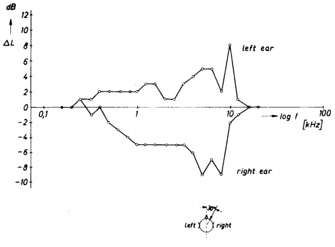
Figure 7.21: Simulation of the directional characteristic of the human head related to the sound incident direction (30°). Reproduced from Plenge G, 1974. 257(fig8)
