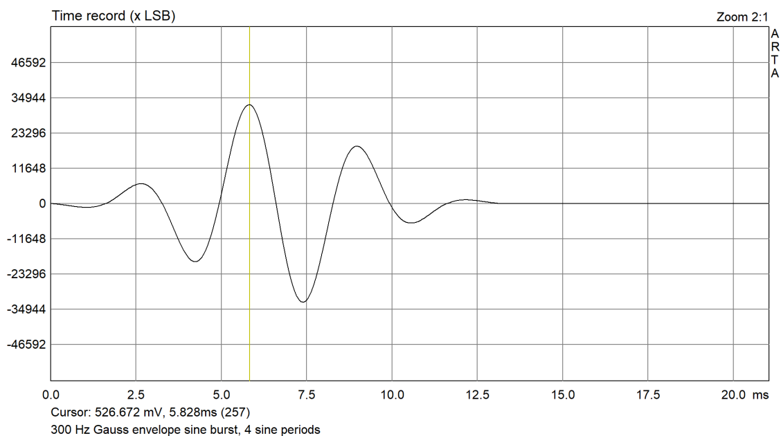
Figure 3.2: POL3 test signal, a 300 Hz Gauss envelope tone burst, 4 sine periods. Zoom 2:1
