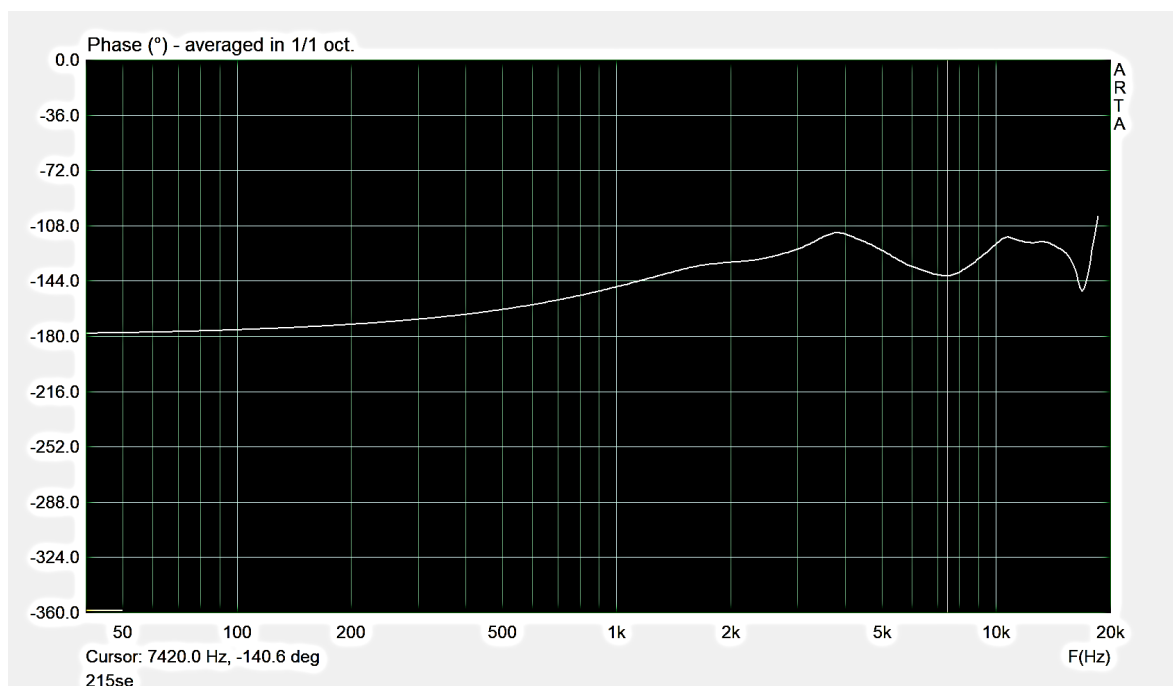
Figure 7.8: Earphone #1 phase estimate (note Phase range)
