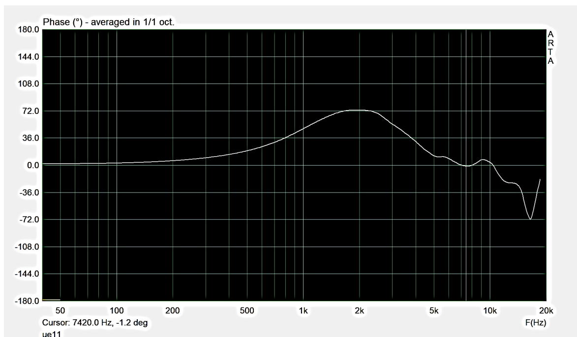
Figure 7.16: Earphone #9 phase estimate
