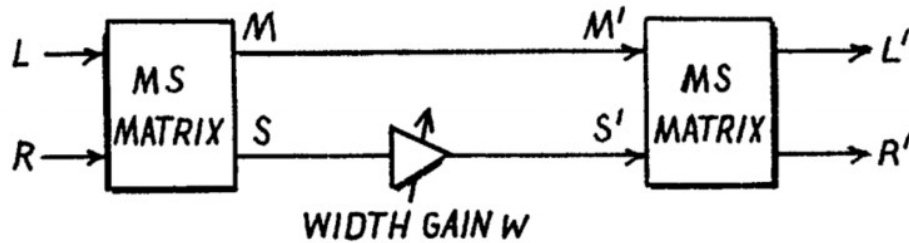
Figure 2.5: Schematic of a width control for amplitude stereophony. The “sum” channels are here denoted as MID signals M and M' , the “difference” channels denoted as S and S' . Reproduced from Gerzon MA, 1992. 98(fig2)
